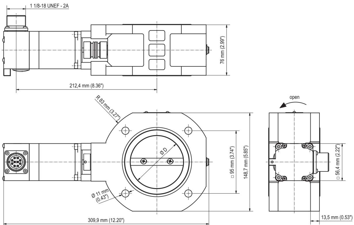
P/N 30.43.140-D-HT
