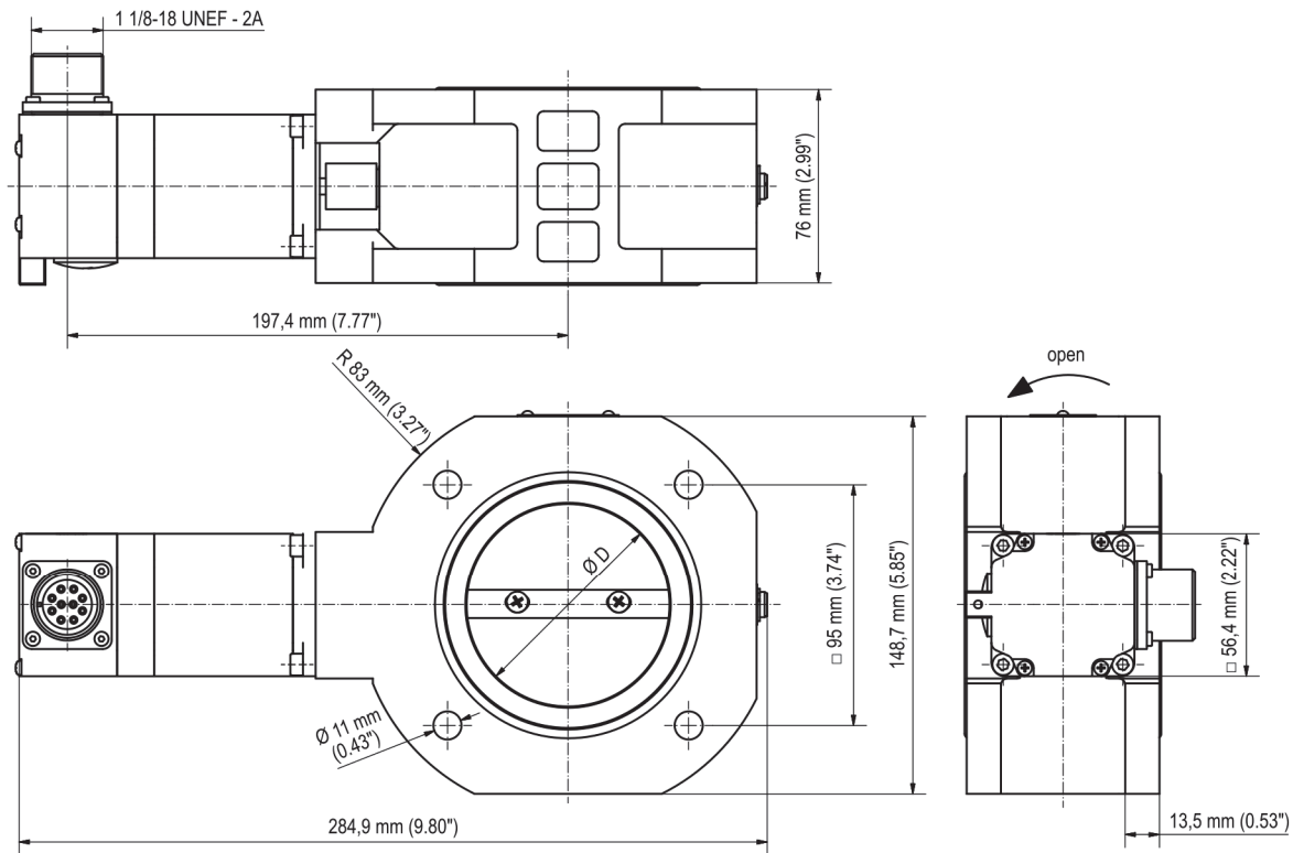
P/N 30.43.140-D-HT
