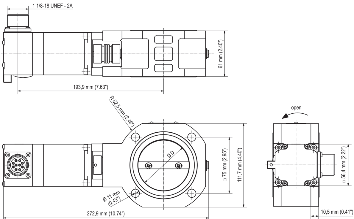
P/N 30.43.100-D-HT
