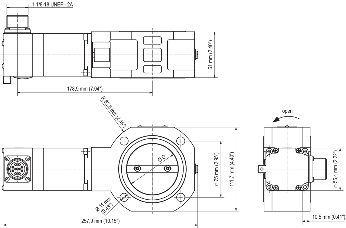
P/N 30.43.100-D
