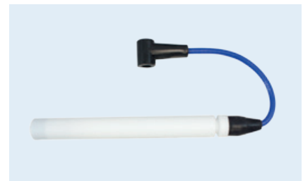
PolyMot™ spark plug lead with embedded groove for safety flange
