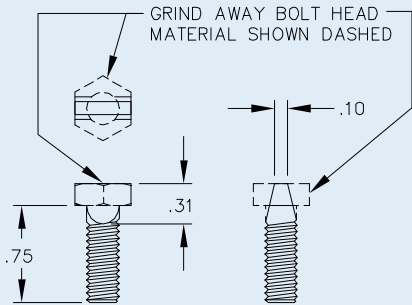
FABRICATE RESET PIN USING 1/4-20 X 3/4 INCH LONG FERROUS HEX BOLT TO DIMENSIONS SHOWN.
