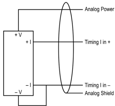
Vier-Draht-Transmitter
